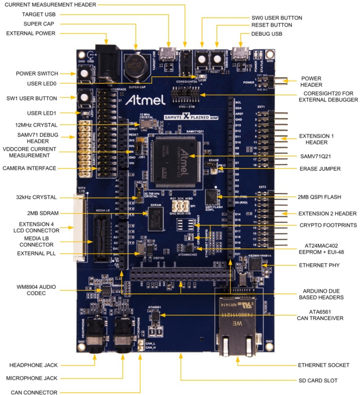
Figure 1-1 SAM V71 Xplained Ultra Evaluation Kit Overview
